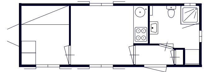
wagen 27 250x780
