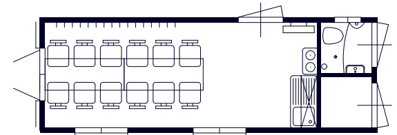
wagen 21 215x650
