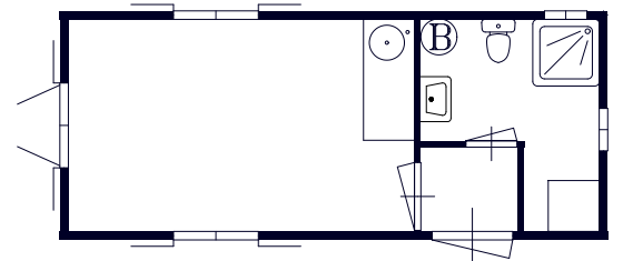
wagen 24 250x650
