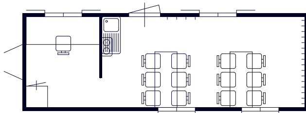
wagen 25 250x780
