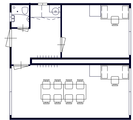
schakel 3 2 units 290x650
